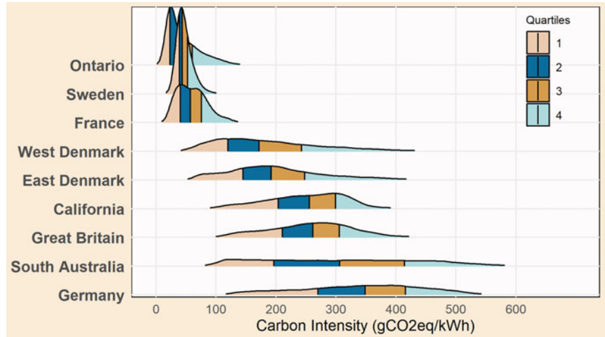
Fig. 6.2 Carbon intensity of electricity consumption 2017–2021. Source @GrantChalmers
