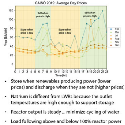
Fig. 6.16 Natrium flexible power output diagram. Storage moves nuclear out of a solely baseload role, allowing greater utilization of renewables. Source TerraPower
